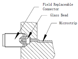
glass bead Transitions to Microstrip and Stripline Circuits
