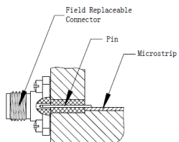
Launch Pin & Dielectric Transitions to Microstrip and Stripline Circuits *refer to combination type connector
