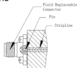
Pin/Tab Transitions to Microstrip and Stripline Circuits *refer to combination type connector
